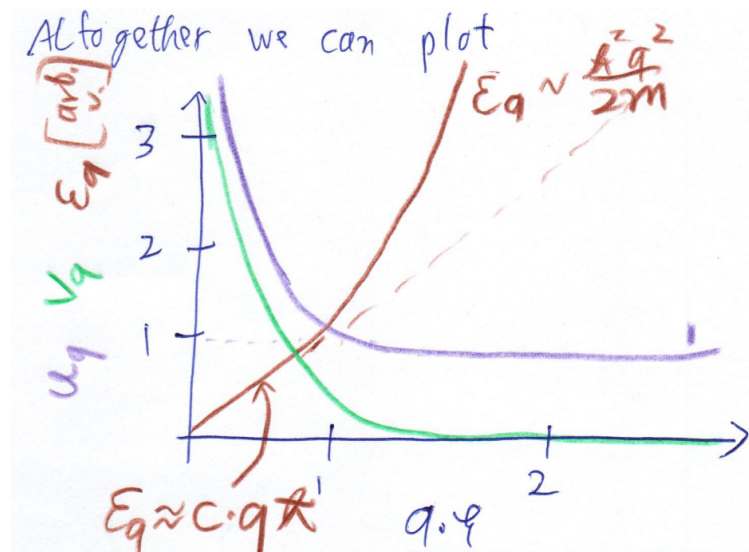
left: Combined plot of Bogoliubov energy \varepsilon_q (3.71) (brown), particle amplitude \bar{u}_q (violet) and hole amplitude \bar{v}_q (green) (3.72).
