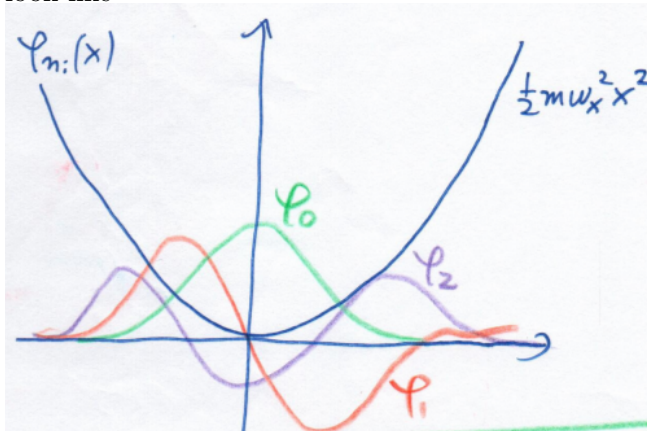
left: Sketch of 1D harmonic oscillator potential and the first few eigenstates
