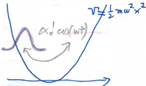
top: Coherent state Gaussian oscillating in a harmonic trap
